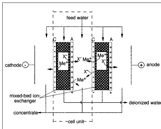
Figure 10. Electrodeionization process.
